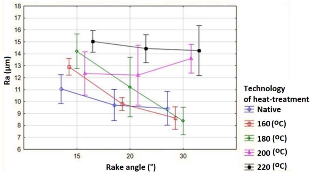
Figure 5: Multifactor analysis of variance of surface roughness dependence on angular geometry for tool set 1
