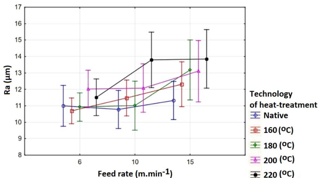
Figure 10: Multifactor analysis of variance of surface roughness dependence on feed rate for tool set 3
