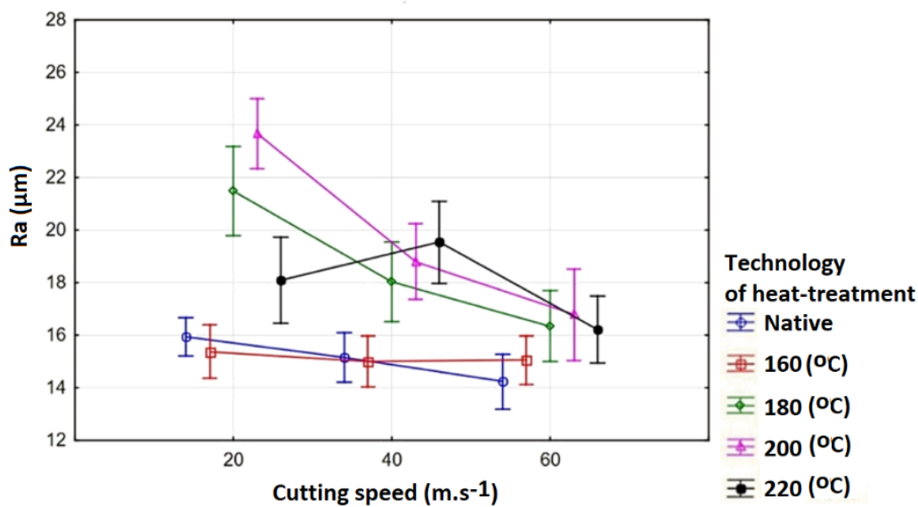
Figure 11: Multifactor analysis of variance of surface roughness dependence on cutting speed for tool set 2
