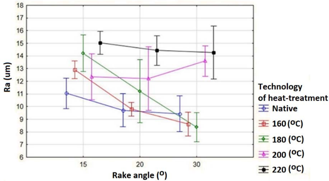
Figure 7: Multifactor analysis of variance of surface roughness dependence on angular geometry for tool set 3
