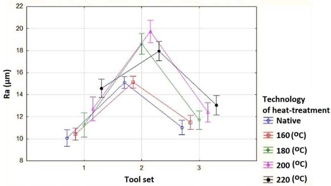
Figure 4: Effect of heat-treatment technology and tool set on surface roughness
