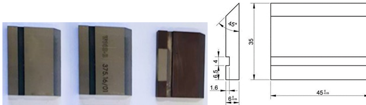
Figure 1: Changeable milling knives and their dimensions
