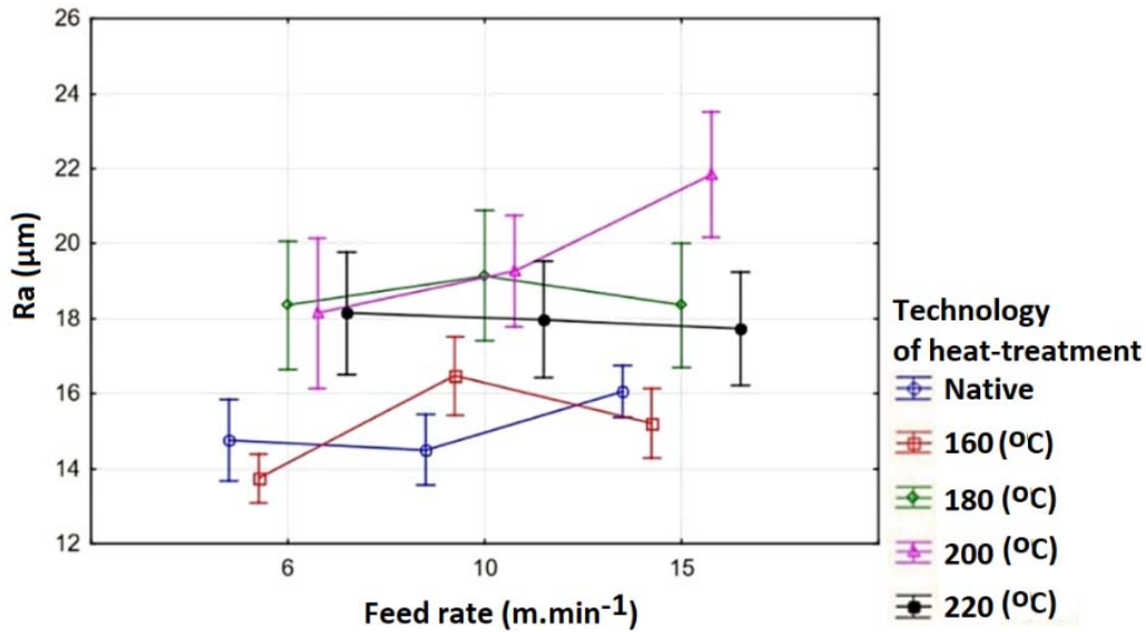
Figure 9: Multifactor analysis of variance of surface roughness dependence on feed rate for tool set 2
