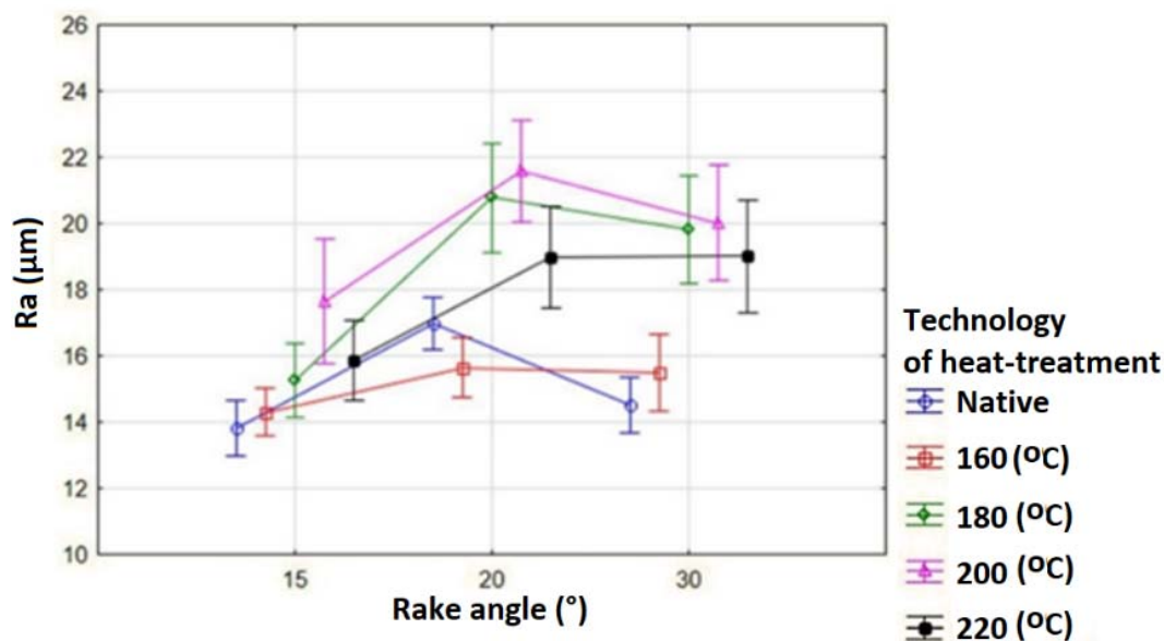
Figure 6: Multifactor analysis of variance of surface roughness dependence on angular geometry for tool set 2
