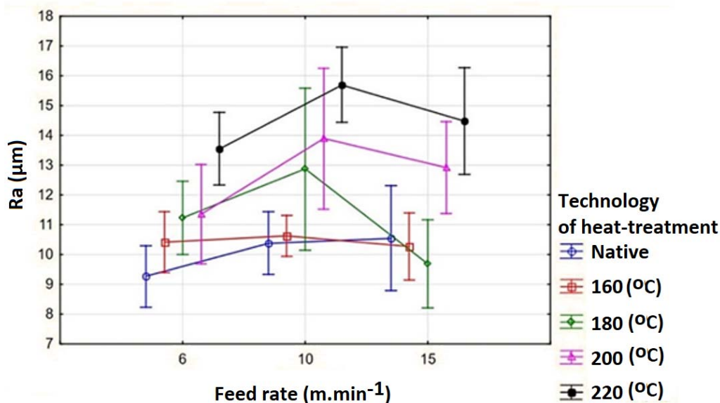
Figure 8: Multifactor analysis of variance of surface roughness dependence on feed rate for tool set 1
