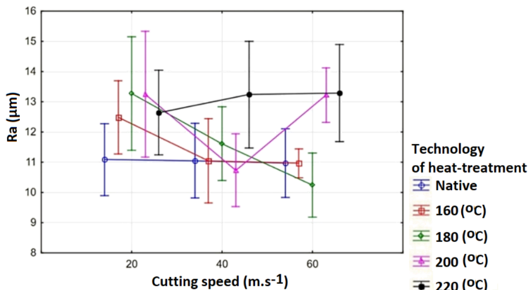
Figure 12: Multifactor analysis of variance of surface roughness dependence on cutting speed for tool set 3
